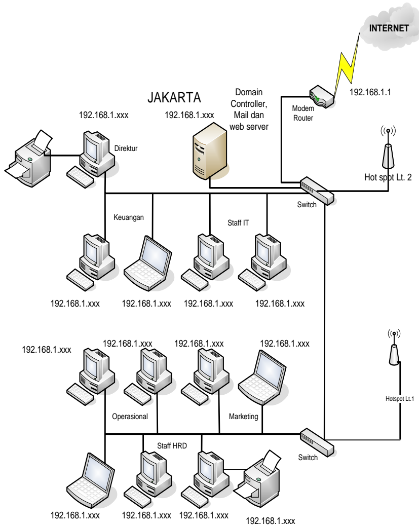
Gambar 2. Skema Jaringan PT. Ehibition Network Indonesia
